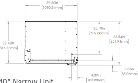
40" Narrow Unit
